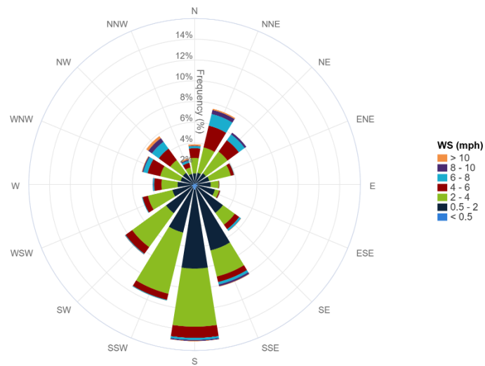
7-Day Wind Rose Plot [From 08/14/2026 00:00 to 08/20/2026 23:59]
