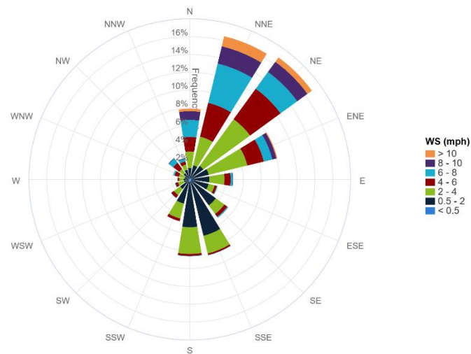
7-Day Wind Rose Plot [From 08/22/2025 00:00 to 08/28/2025 23:59]
