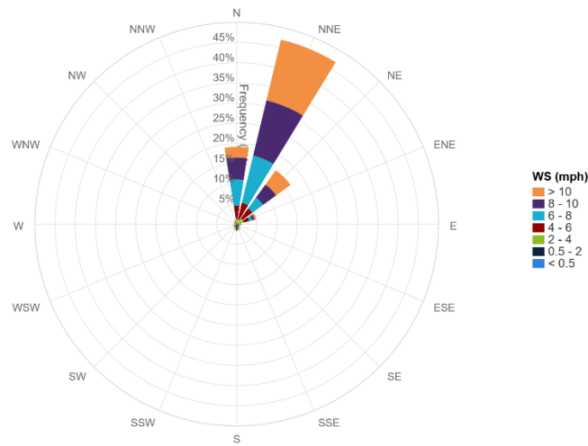
7-Day Wind Rose Plot [From 08/01/2025 00:00 to 08/07/2025 23:59]
