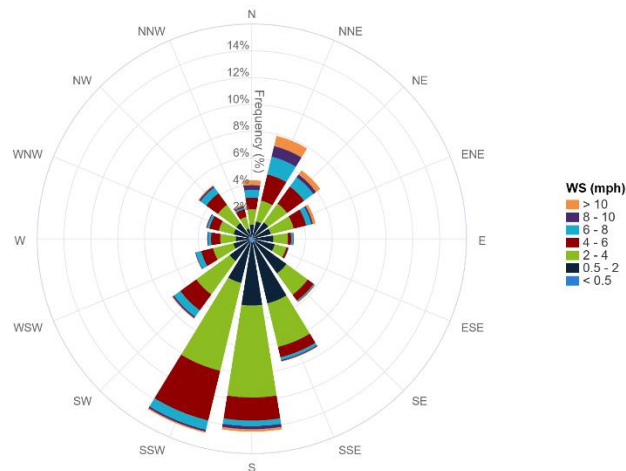
7-Day Wind Rose Plot [From 07/25/2025 00:00 to 07/31/2025 23:59]
