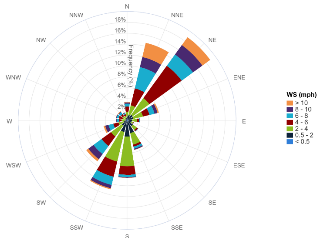
7-Day Wind Rose Plot [From 07/18/2025 00:00 to 07/24/2025 23:59]
