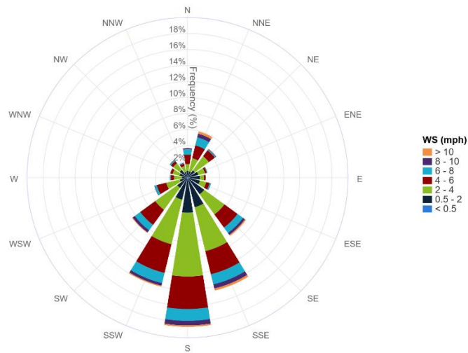
7-Day Wind Rose Plot [From 07/11/2025 00:00 to 07/17/2025 23:59]
