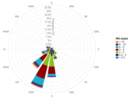
7-Day Wind Rose Plot [From 6/06/2025 00:00 to 6/12/2025 23:59]
