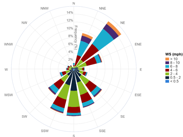
7-Day Wind Rose Plot [From 5/09/2025 00:00 to 5/15/2025 23:59]
