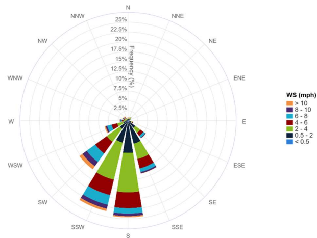
7-Day Wind Rose Plot [From 5/02/2025 00:00 to 5/08/2025 23:59]
