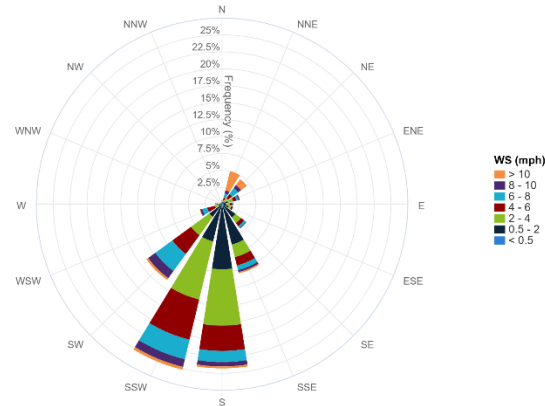
7-Day Wind Rose Plot [From 4/25/2025 00:00 to 5/01/2025 23:59]
