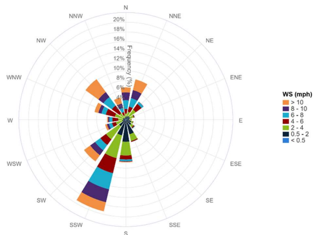
7-Day Wind Rose Plot [From 4/11/2025 00:00 to 4/17/2025 23:59]
