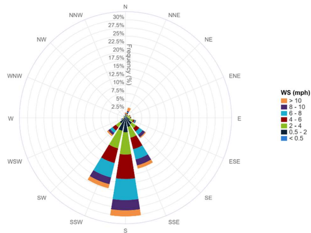
7-Day Wind Rose Plot [From 3/28/2025 00:00 to 4/03/2025 23:59]
