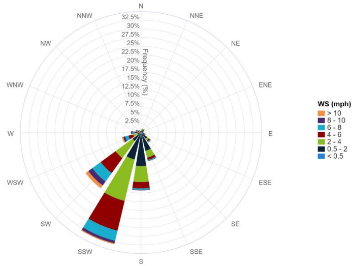
7-Day Wind Rose Plot [From 1/24/2025 00:00 to 1/30/2025 23:59]
