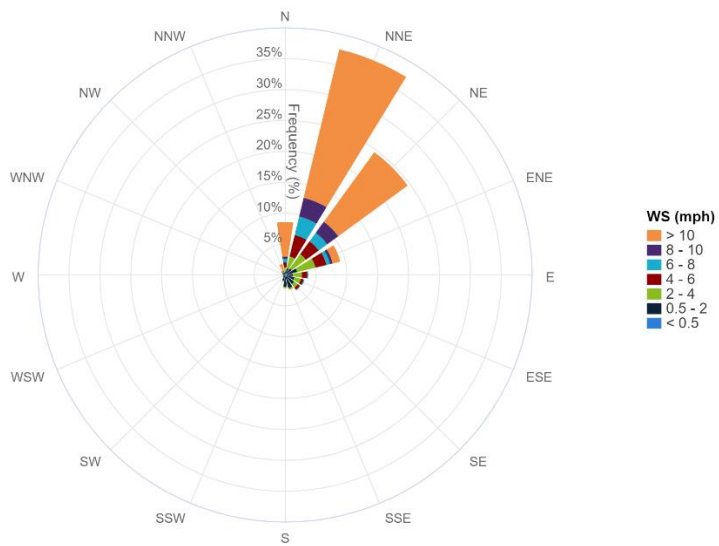
7-Day Wind Rose Plot [From 09/13/2024 00:00 to 09/19/2024 23:59]
