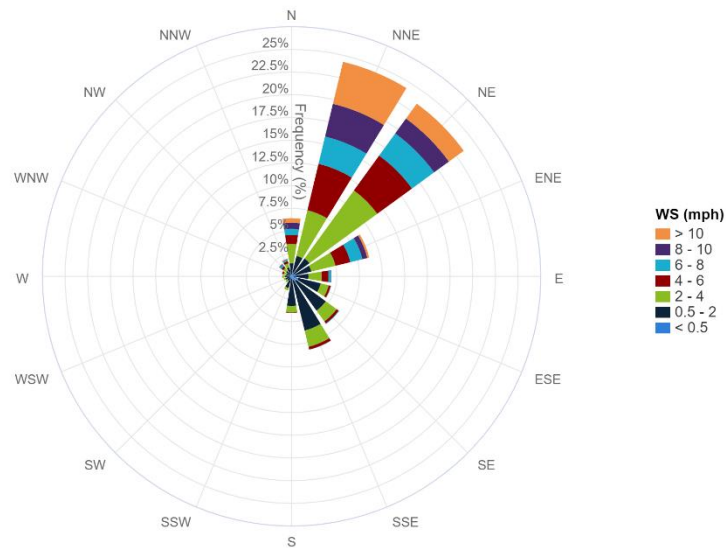
7-Day Wind Rose Plot [From 09/06/2024 00:00 to 09/12/2024 23:59]
