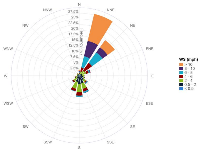
7-Day Wind Rose Plot [From 08/30/2024 00:00 to 09/05/2024 23:59]
