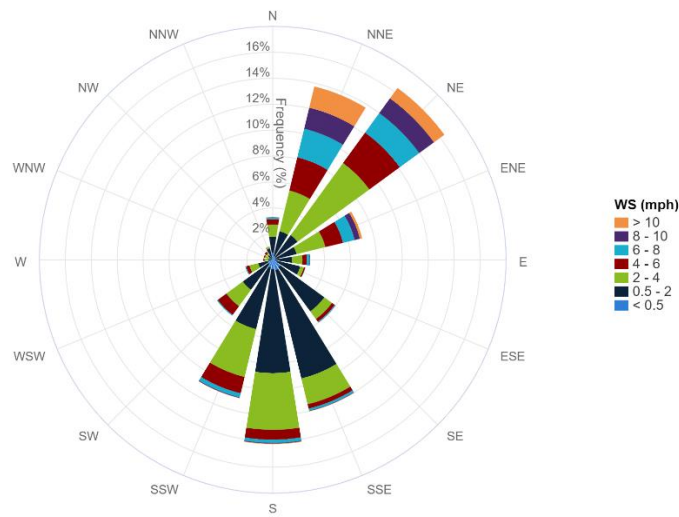
7-Day Wind Rose Plot [From 08/23/2024 00:00 to 08/29/2024 23:59]
