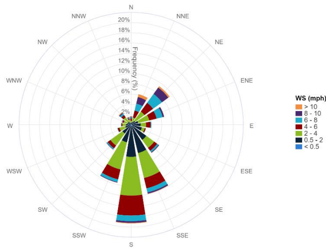
7-Day Wind Rose Plot [From 07/26/2024 00:00 to 08/01/2024 23:59]
