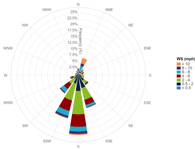
7-Day Wind Rose Plot [From 07/05/2024 00:00 to 07/11/2024 23:59]
