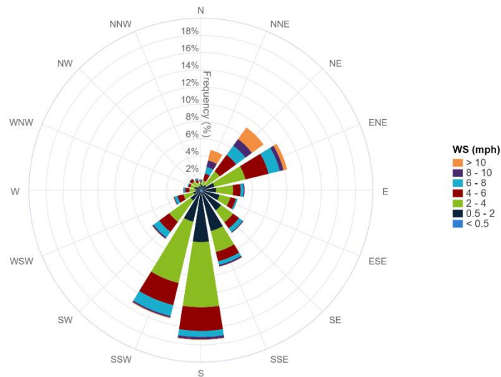
7-Day Wind Rose Plot [From 06/28/2024 00:00 to 07/04/2024 23:59]
