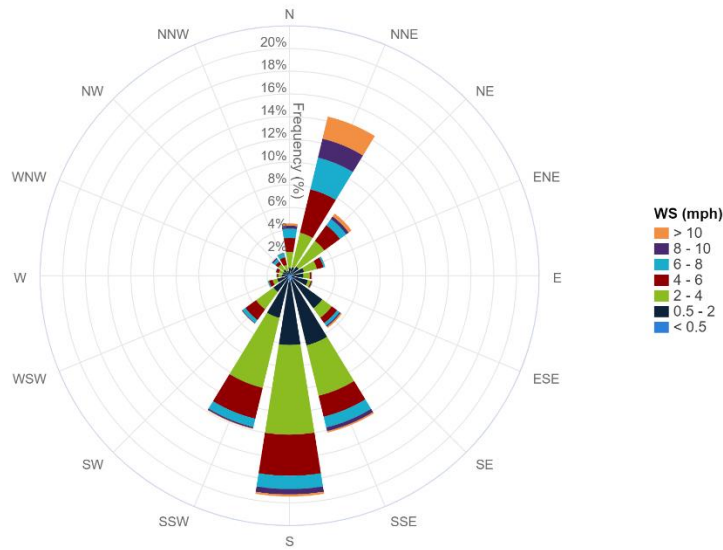
7-Day Wind Rose Plot [From 06/21/2024 00:00 to 06/27/2024 23:59]
