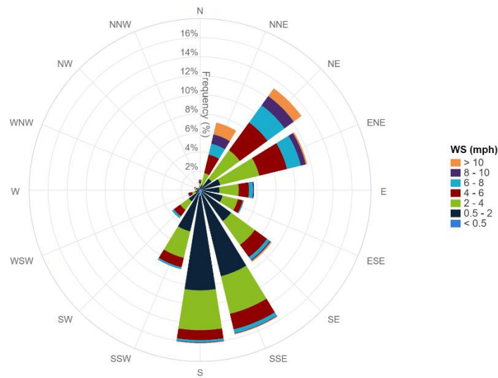
7-Day Wind Rose Plot [From 06/14/2024 00:00 to 06/20/2024 23:59]
