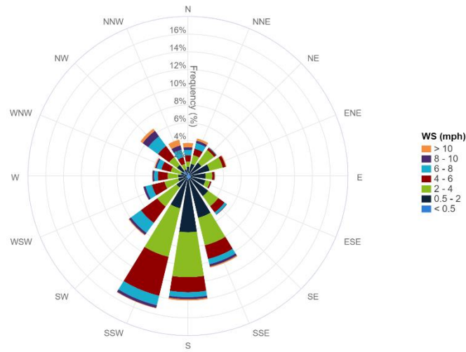
7-Day Wind Rose Plot [From 05/10/2024 00:00 to 05/16/2024 23:59]
