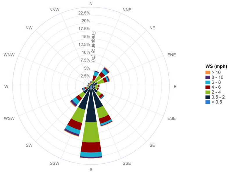
7-Day Wind Rose Plot [From 04/26/2024 00:00 to 05/02/2024 23:59]
