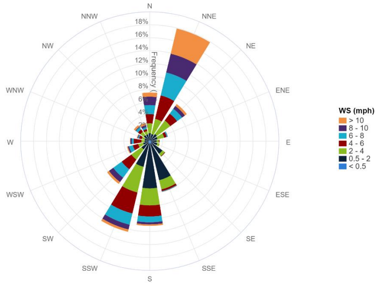
7-Day Wind Rose Plot [From 04/19/2024 00:00 to 04/25/2024 23:59]
