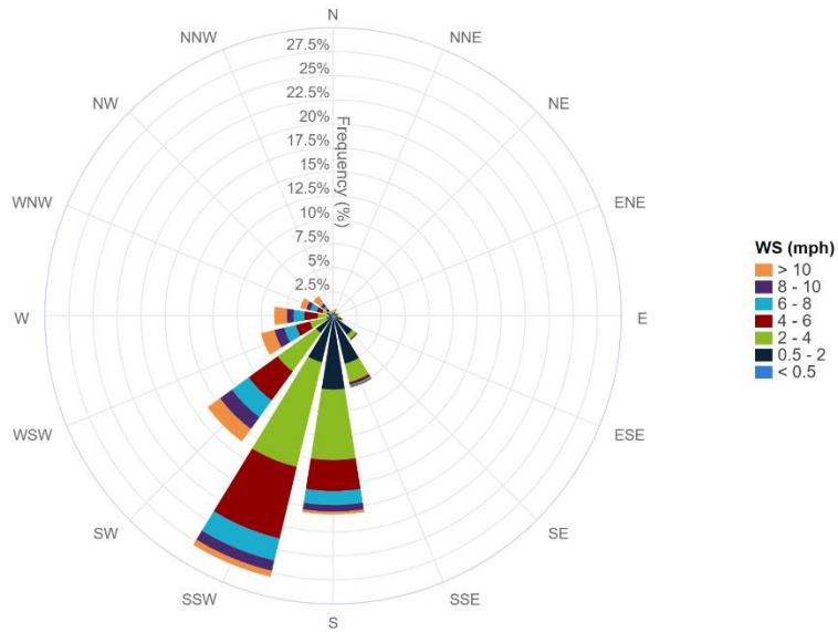
7-Day Wind Rose Plot [From 04/12/2024 00:00 to 04/18/2024 23:59]
