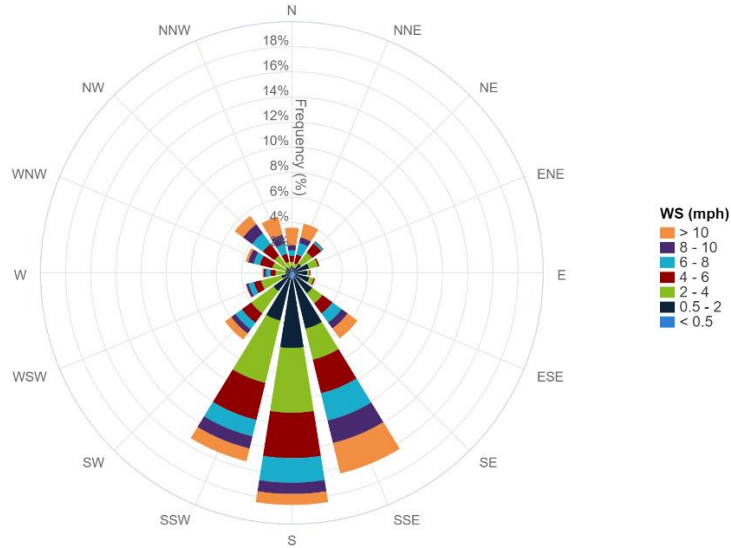
7-Day Wind Rose Plot [From 04/05/2024 00:00 to 04/11/2024 23:59]
