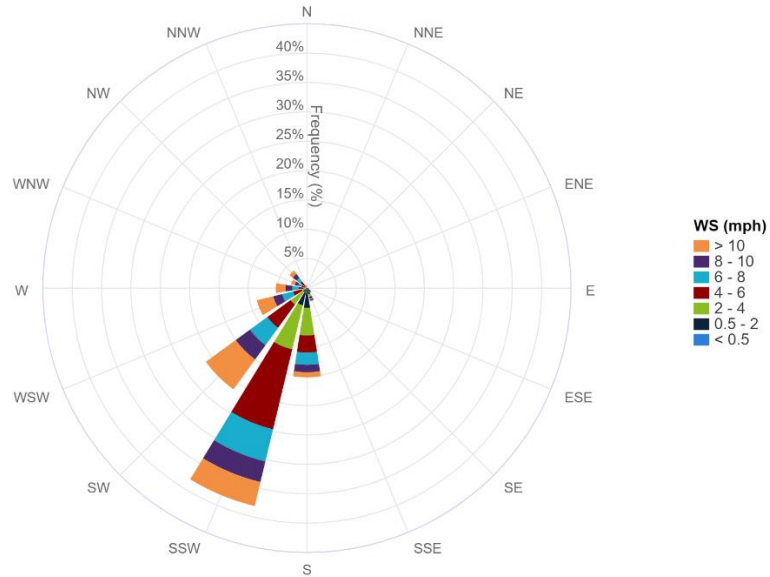
7-Day Wind Rose Plot [From 03/29/2024 00:00 to 04/04/2024 23:59]
