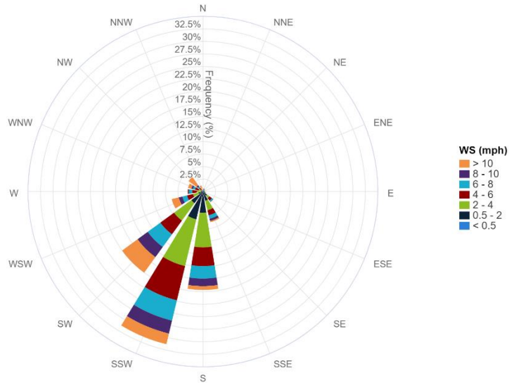
7-Day Wind Rose Plot [From 02/09/2024 00:00 to 02/15/2024 23:59]
