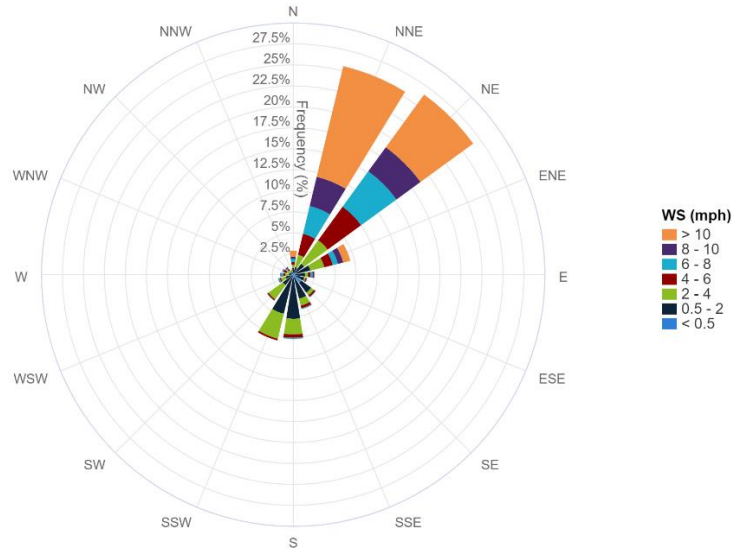
7-Day Wind Rose Plot [From 02/02/2024 00:00 to 02/08/2024 23:59]
