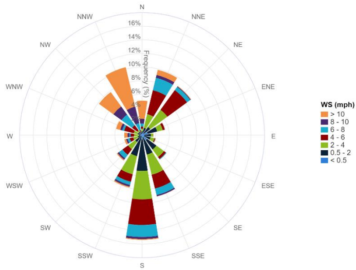
7-Day Wind Rose Plot [From 01/19/2024 00:00 to 01/25/2024 23:59]
